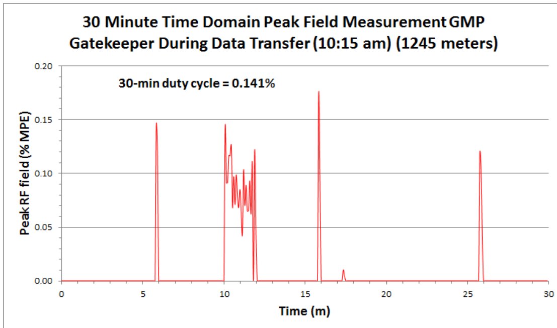
Figure 38. A 30-minute time domain measurement of peak RF fields near the base of a GMP Gatekeeper (site 8) during a scheduled transmission of data accumulated from 1245 end point meters.
